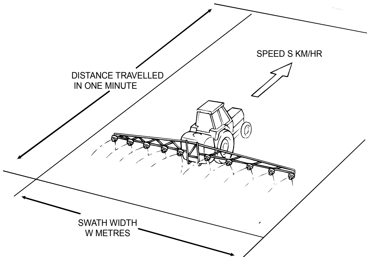
Figure 9. Coverage of sprayer
