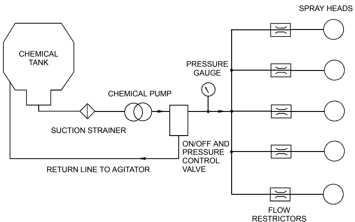
Figure 8. Typical configuration of chemical feed to heads
