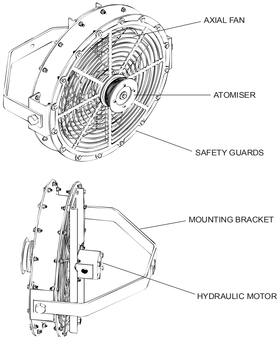
Figure 1. Turbofan spray head
